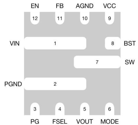
Figure 1. 12-Lead Plastic QFN ( Top view: 2mmx3mm)
