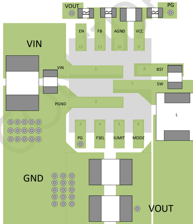
Figure 35. PCB Layout Example
