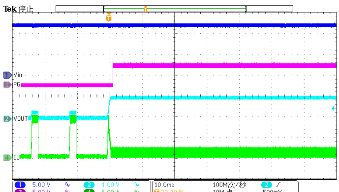
Figure 22. Over Current Release (hard short to 1A) ILIMIT=10A
