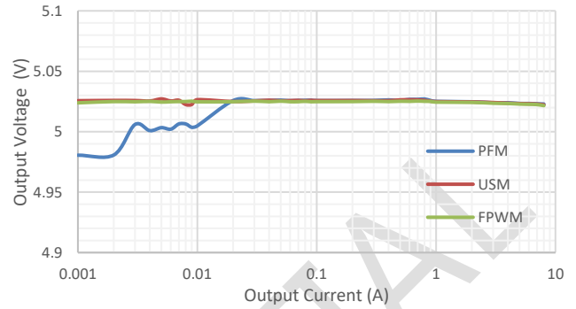
Figure 9. Load Regulation, Vout=5V, Fsw=400kHz
