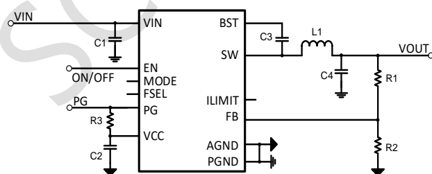
2.9V-16V, Synchronous Buck Converter
