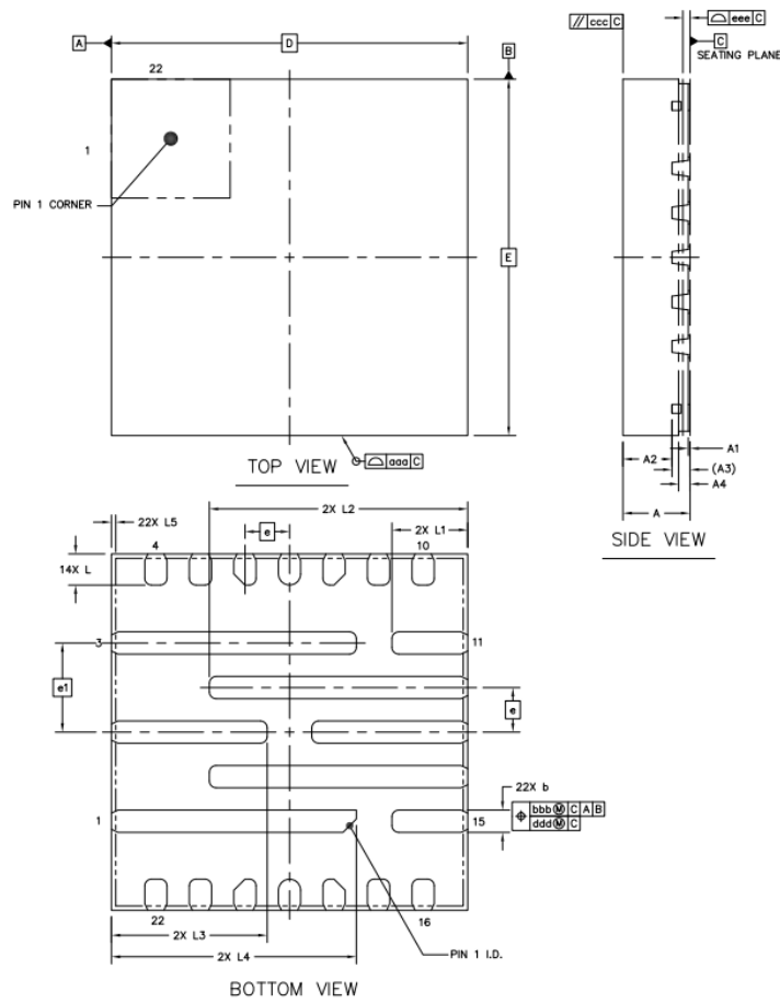
FCQFN-22L (4x4) Package Outline Dimensions
