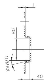
SECTION Y-Y
