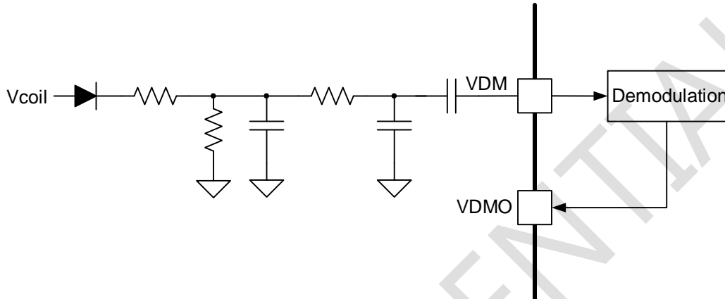
Figure 10. Envelope Detector
