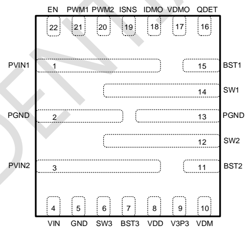
Figure 1. Top view 22-Lead QFN 4mm*4mm
