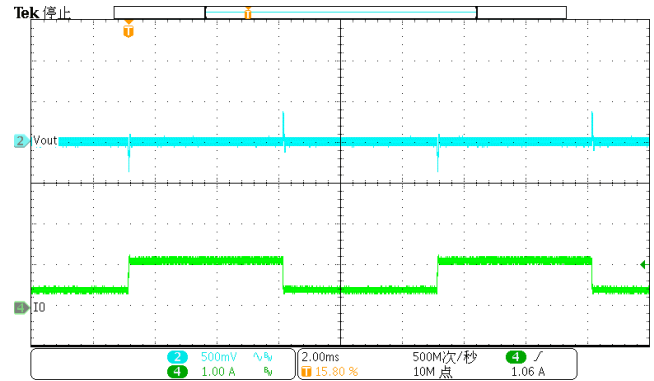
Figure 18. Load Transient (0.38A-1.12A, 1.6A/us)
