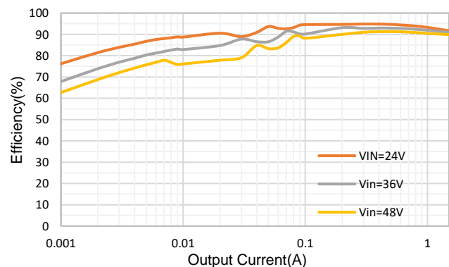
Efficiency, Vout=12V
