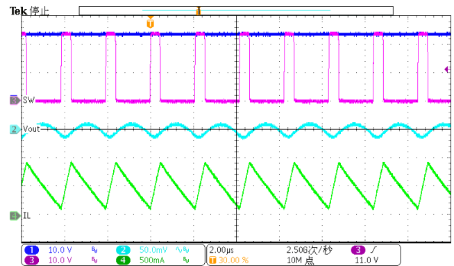
Figure 20. Output Ripple (ILOAD=0.5A)
