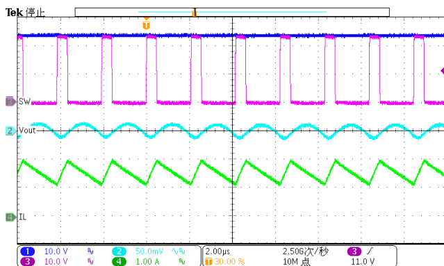
Figure 21. Output Ripple (ILOAD=1.5A)
