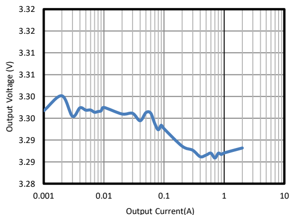
Figure 5. Load Regulation (VIN=12V, VOUT=3.3V)
