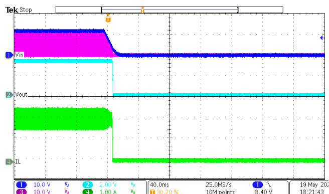
Figure 18. Power down
