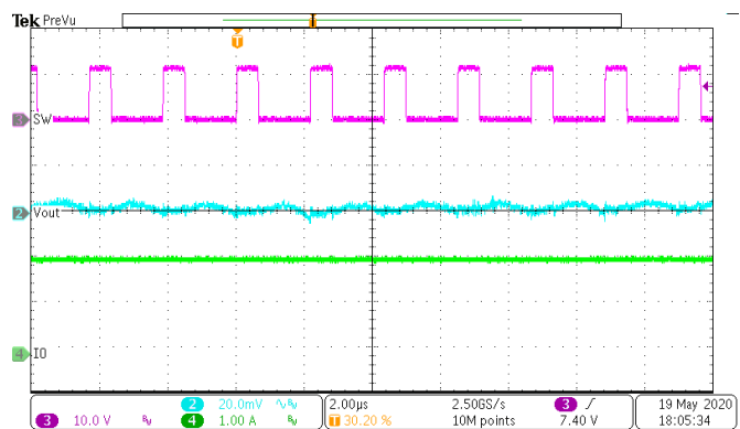
Figure 21. SW and Vout Ripple (Iout=2A)
