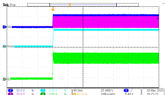
Figure 17. Power up
