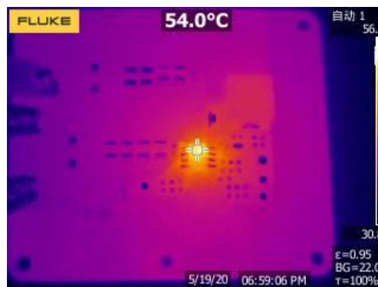
Figure 22. Thermal, 3.3Vout/2A
