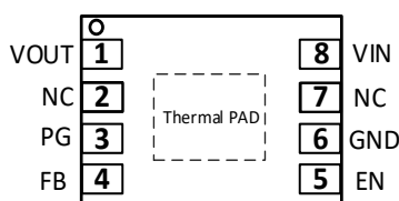
SCT71005A02DTDR DFN2x3-8 Package
