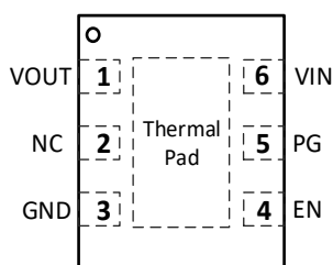
SCT71005FxxDVAR DFN2x2-6 Package
