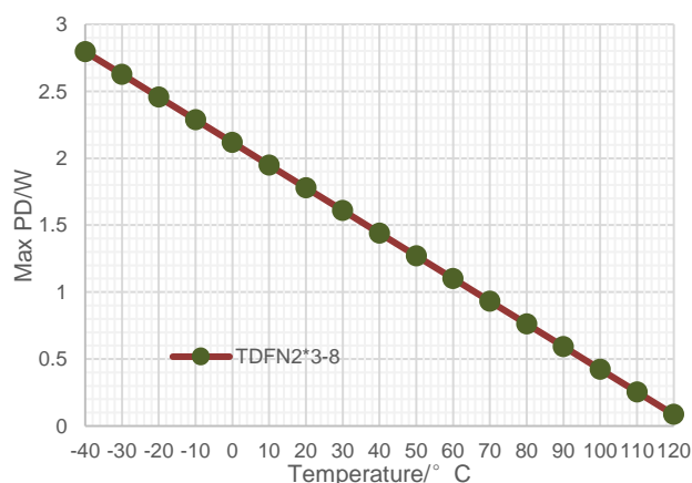
Figure 31. Maximum Allowed Power Dissipation vs Ambient Temperature, DFN2x3-8, T_J \leq 125^\circ\text{C}
