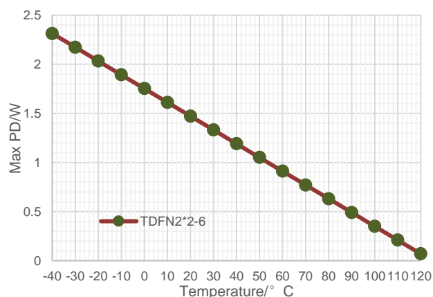
Figure 30. Maximum Allowed Power Dissipation vs Ambient Temperature, DFN2x2-6, T_J \leq 125^\circ\text{C}
