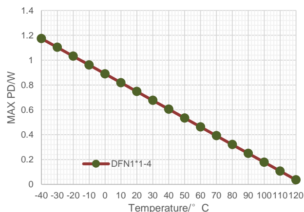
Figure 33. Maximum Allowed Power Dissipation vs Ambient Temperature, DFN1x1-4, T_J \leq 125^\circ\text{C}
