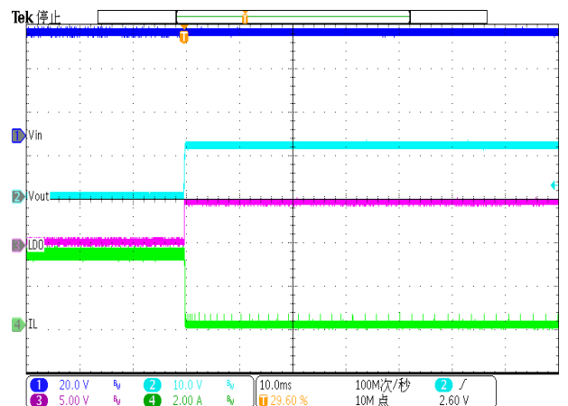
Figure 22. DC-DC Over Current Release
