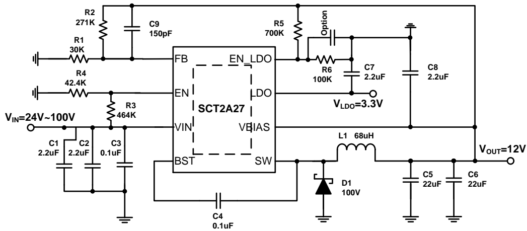
Figure 16. SCT2A27 Design Example, BUCK 12V Output , LDO 3.3V Output
