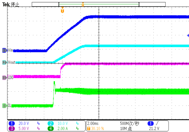
Figure 17. Power up (Iload=2A)
