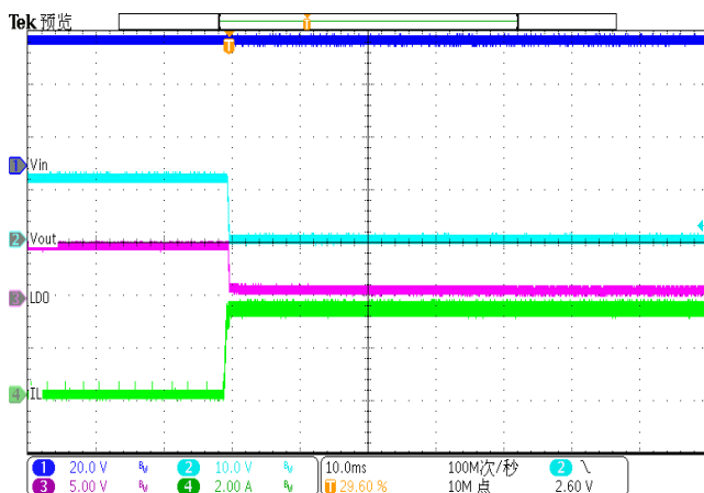
Figure 21. DC-DC Over Current Protection
