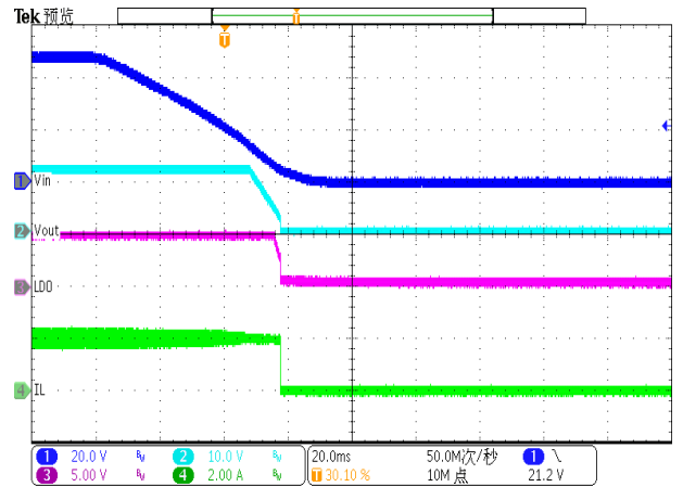
Figure 18. Power down (Iload=2A)
