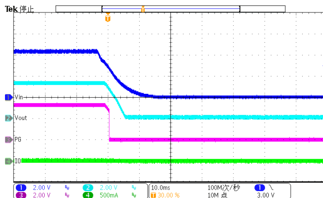
Figure 30. Power down (Iload=10mA)
