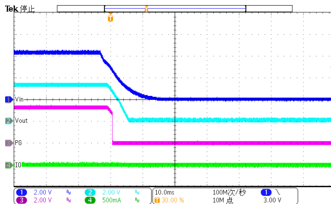
Figure 32. Slow Power down (Iload=10mA)
