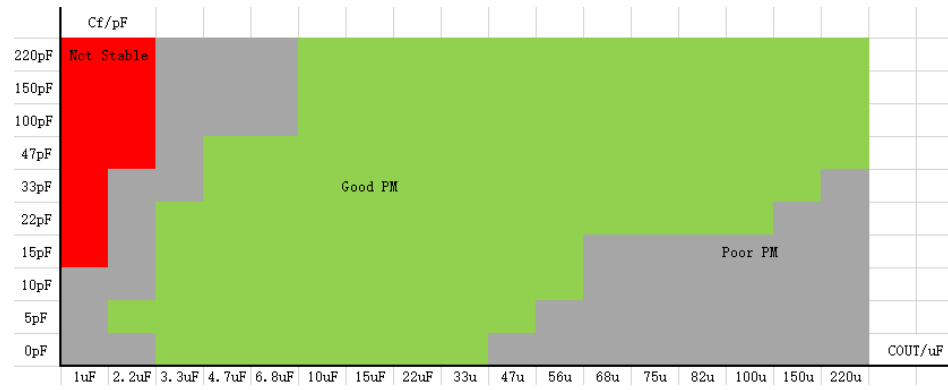
Figure 24. SCT71010A00Q Feed Forward Capacitors recommend( R2=100k\Omega , V_{OUT}=1.8V )
