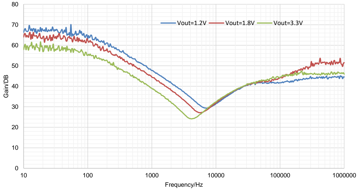
Figure 13. PSRR vs Frequency VIN=4.3V, Cf=33pF, COU=10uF, IOUT=10mA
