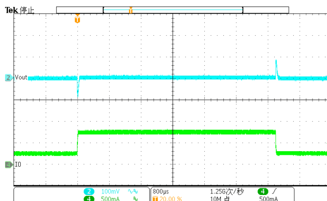
Figure 34. DC-DC Load Transient (250mA-750mA), V_{OUT} = 3.3V
