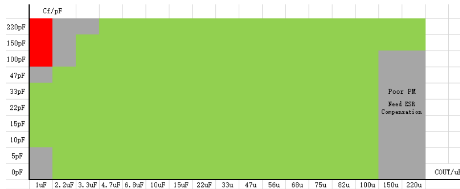
Figure 25. SCT71010A00Q Feed Forward Capacitors recommend( R_2=10k\Omega , V_{OUT}=1.8V )
