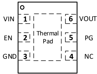
SCT71403FxxAQDVAR DFN2x2-6 Package
