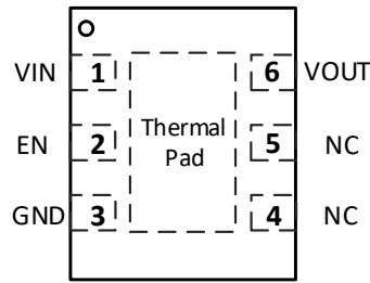
SCT71403FxxQDVAR DFN2x2-6 Package
