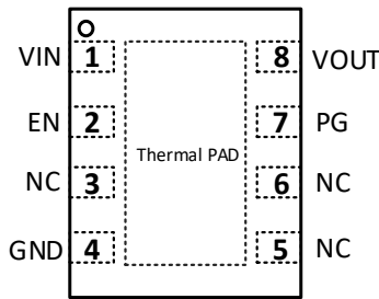
SCT71403FxxQDTBR DFN3x3-8 Package
