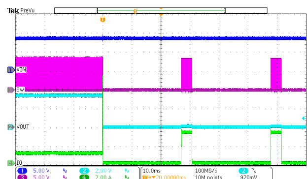
Figure 17. Over Current Protection (1A to hard short)
