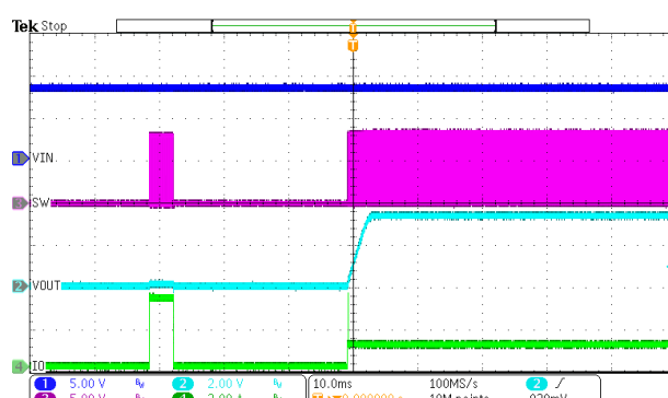
Figure 18. Over Current Release (hard short to 1A)
