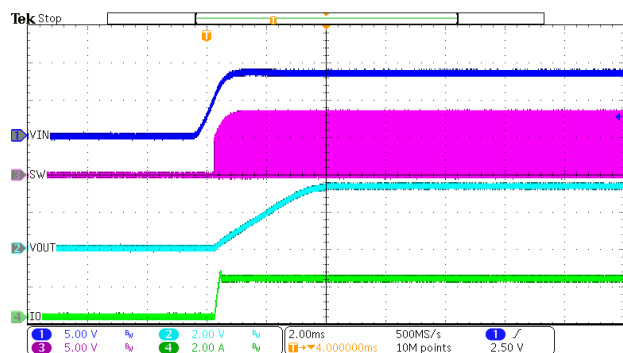
Figure 13. Power up (Iload=2A)
