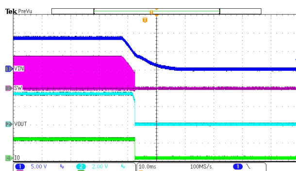
Figure 14. Power down (Iload=2A)
