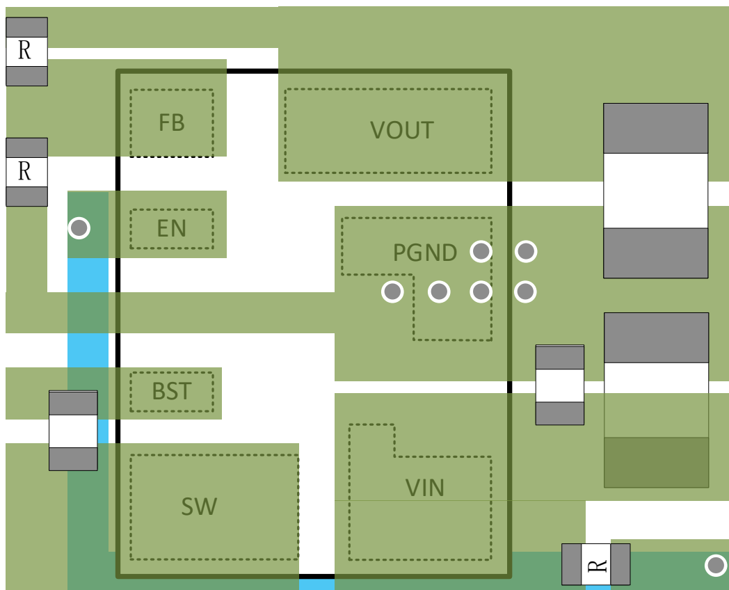
Figure 25. PCB Layout Example
