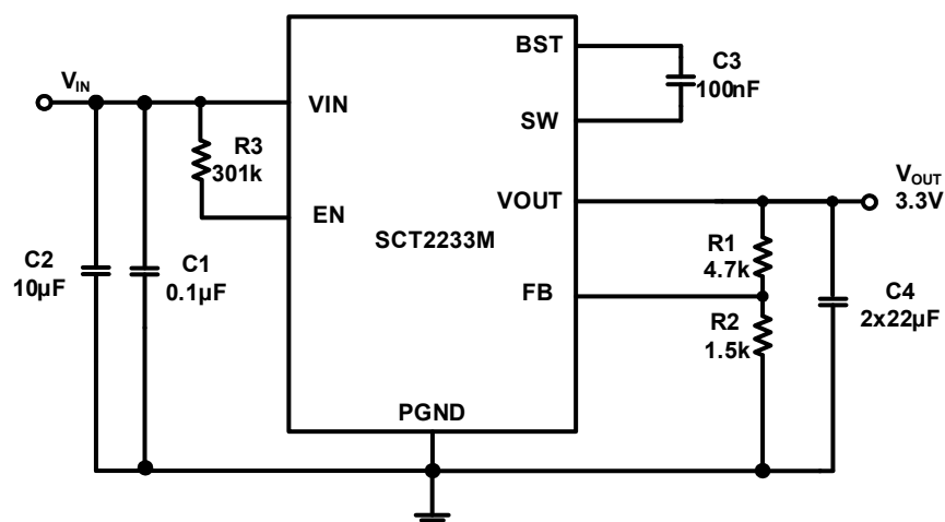
Figure 12. 8.5V Input, 3.3V/2A Output
