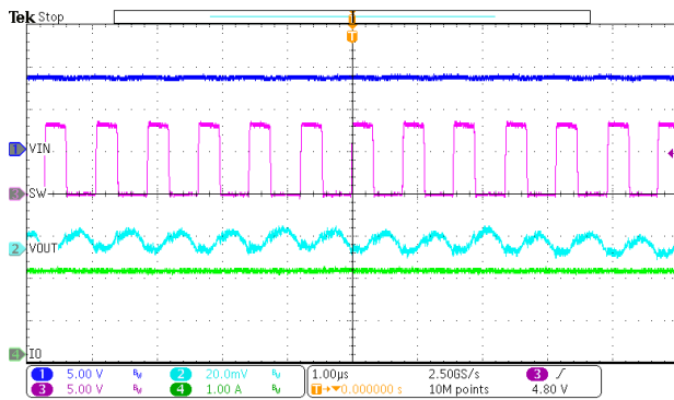
Figure 23. Output Ripple (Iload=2A)
