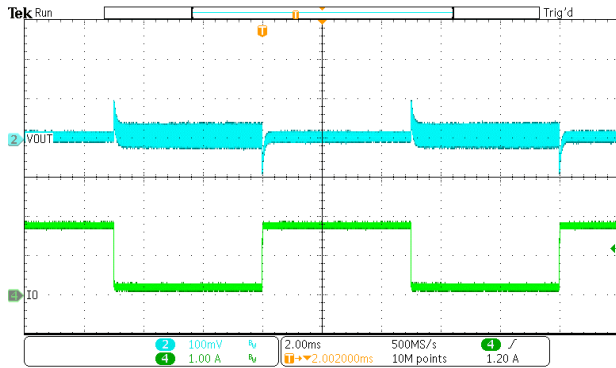
Figure 19. Load Transient (0.2A-1.8A, 0.1A/us)
