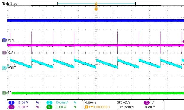
Figure 21. Output Ripple (Iload=0A)
