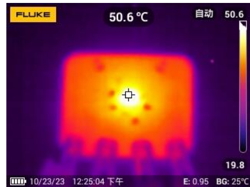
Figure 24 Thermal, 3.3Vout/2A
