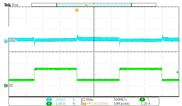
Figure 20. Load Transient (0.5A-1.5A, 0.1A/us)
