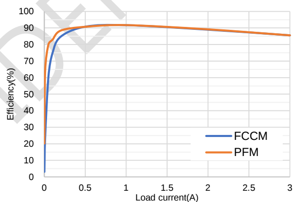
Buck1 Efficiency vs Load Current, V_{OUT1}=3.3V , f_{SW1}=400kHz
