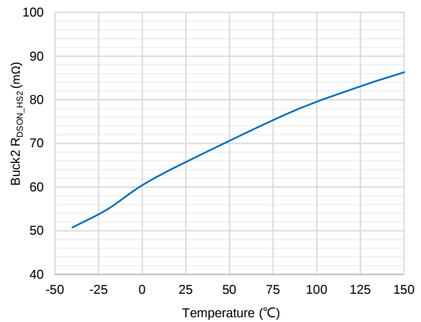
Buck2 R_{DS(on)_HS2} vs. Temperature
