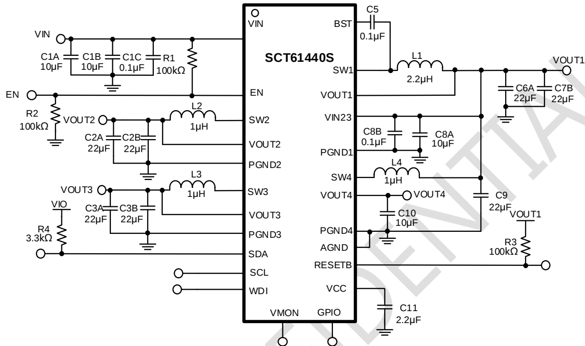
Figure 8. Application Schematic, 3.5V to 36V, PMIC Regulator at 2.2MHz
