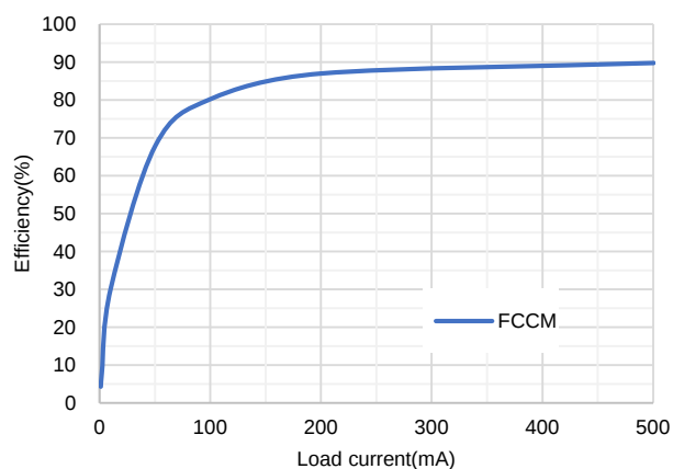
Boost Efficiency vs. Load Current, V_{OUT4}=5V
