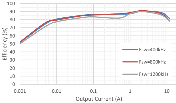
Figure 4. Efficiency at VIN=5V, Vout=1V
