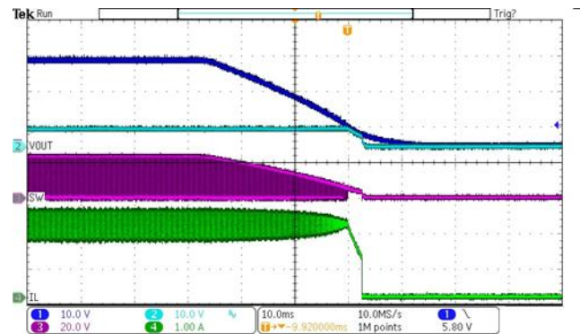
Figure 15. Power Down VIN=24V, VOUT=5V, IOUT=2A
