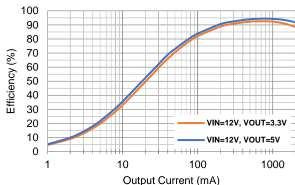
Figure 1. SCT2321 Efficiency, Vin=12V
