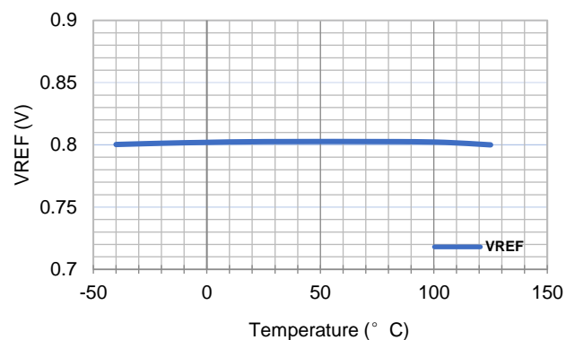
Figure 4. Reference Voltage vs Temperature
