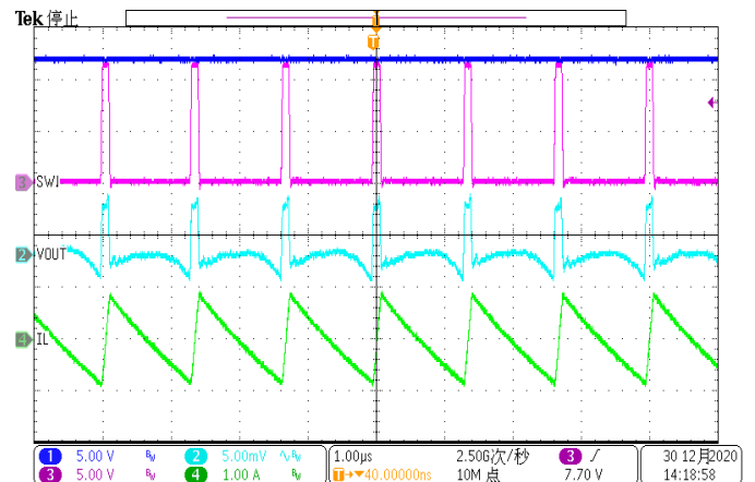
Figure 20. Output Ripple (Iload=0A, FPM)
