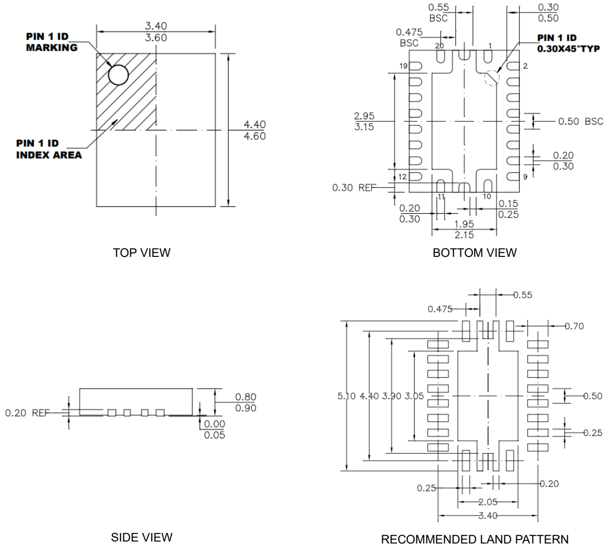
QFN-20L (3.5*4.5) Package Outline Dimensions
