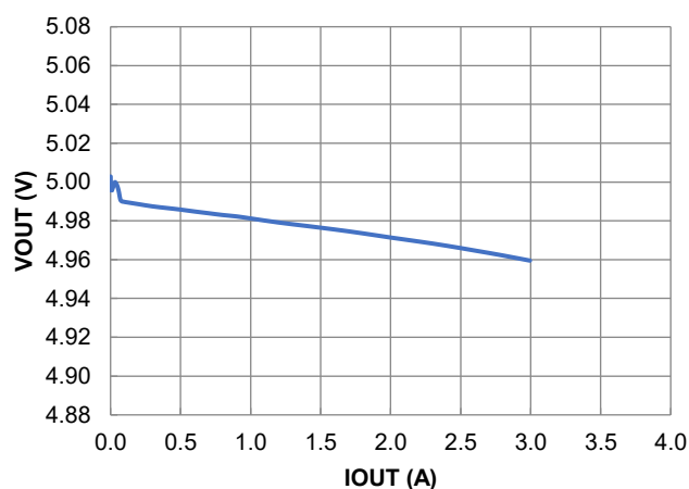
Figure 4. Load Regulation
