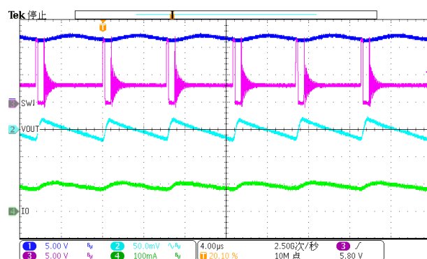
Figure 18. Output Ripple (Iload=0.1A)
