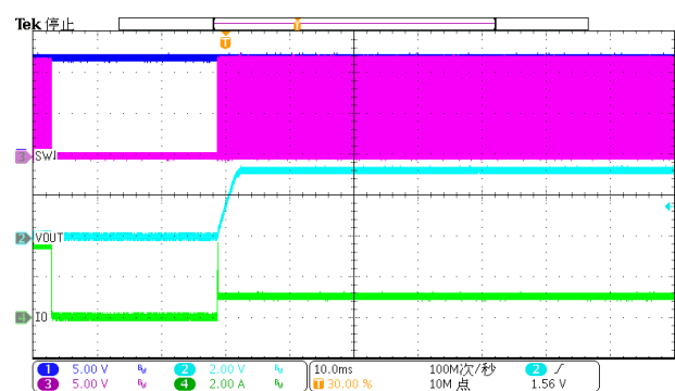
Figure 14. Over Current Release (hard short to 1A)
