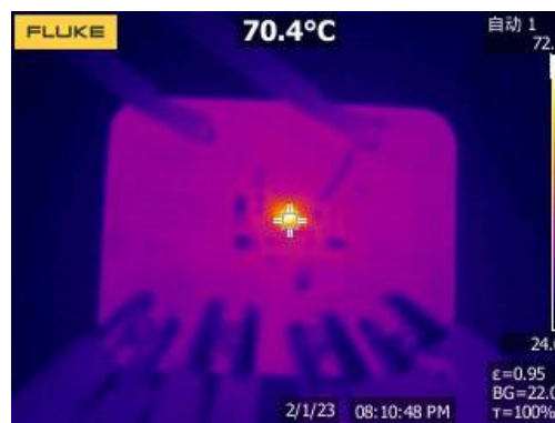
Figure 20. Thermal, 3.3Vout/2A
