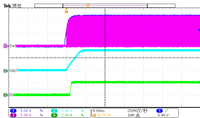
Figure 9. Power up(Iload=2A)
