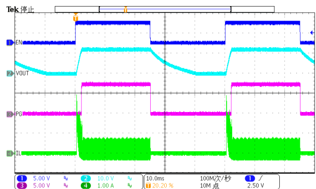
Figure 32. Enable (Iload=0.1A)
