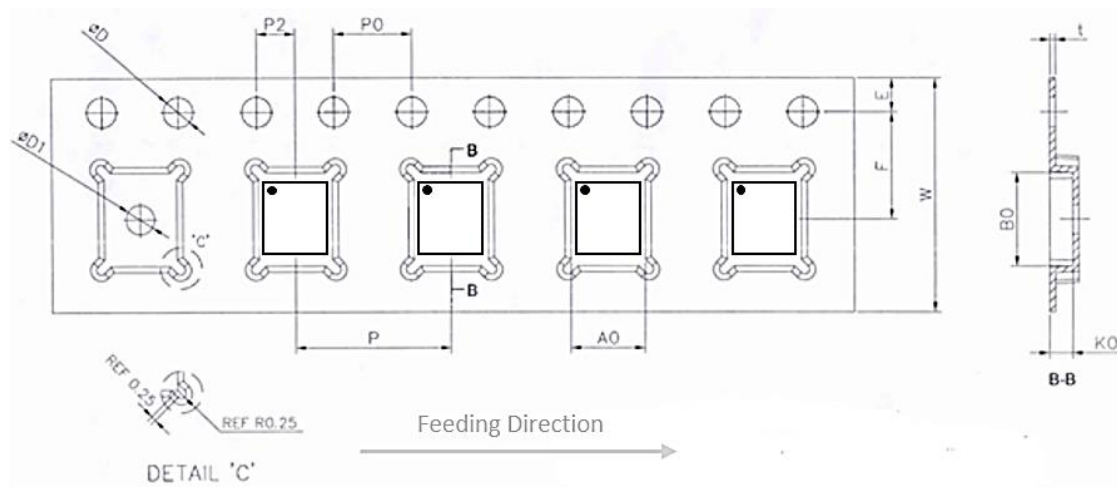
TAPE DIMENSIONS
