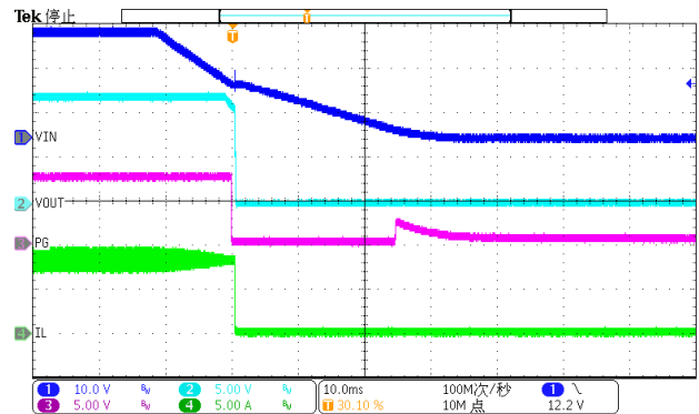
Figure 30. Power down(Iload=8A)
