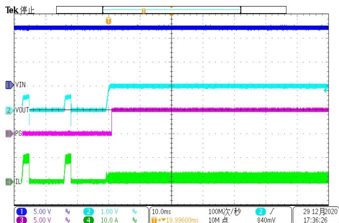
Figure 16. Over Current Release (hard short to 1A)
