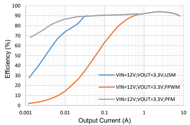
Figure 3. Efficiency vs Iload, Vout=3.3V, fsw=800kHz
