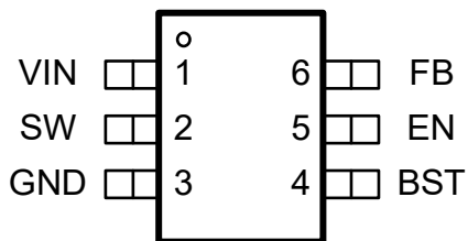
Top View: SOT563 Top View 1.6mm x 1.6mm, Plastic
