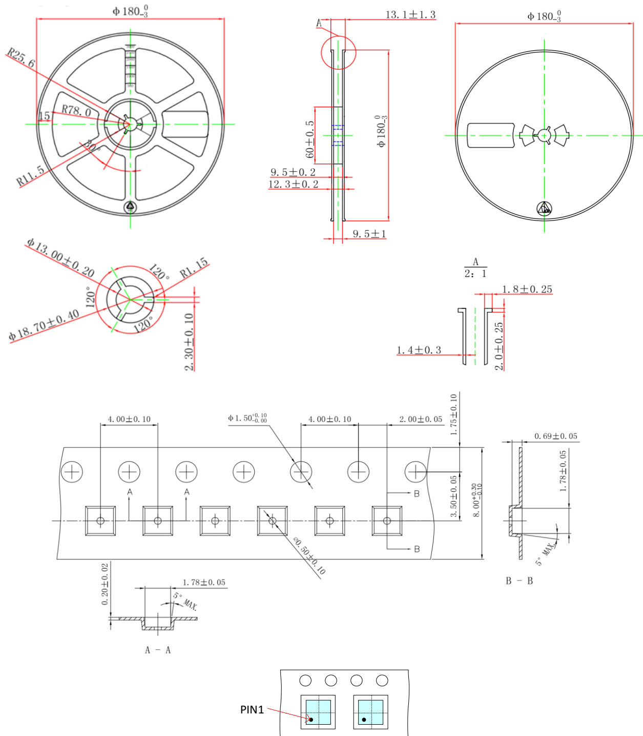
TAPE DIMENSIONS
