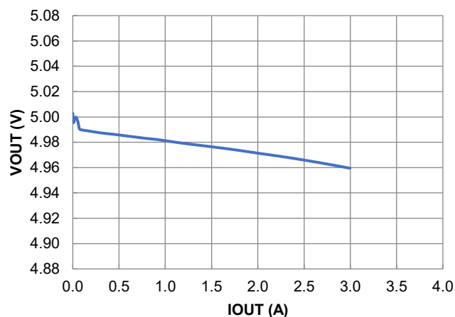
Figure 3. Load Regulation
