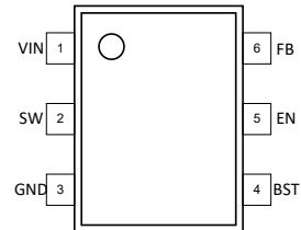
SOT563 Top View (1.6mm x 1.6mm)
