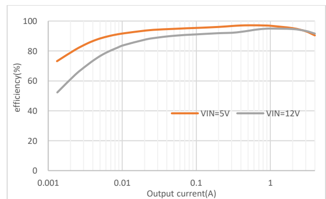
Efficiency, VOUT=3.3V
