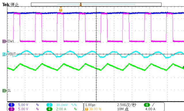
Figure 19. Output Ripple (Iload=4A)
