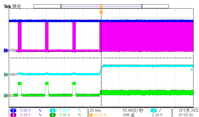
Figure 14. Over Current Release (1A to hard short)
