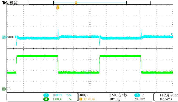
Figure 15. Load Transient (1.5A-3A, 1.6A/us)
