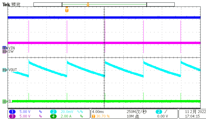
Figure 17. Output Ripple (Iload=0A)
