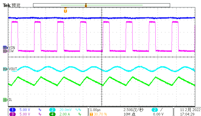
Figure 19. Output Ripple (Iload=3A)
