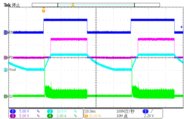
Figure 32. Enable ( I_{load}=0.1A )
