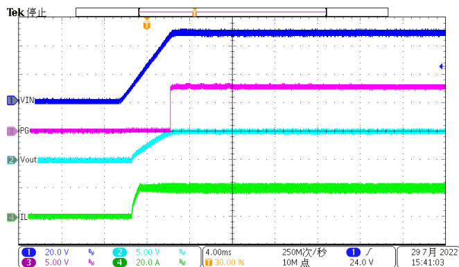
Figure 42. Power up(Iload=20A)
