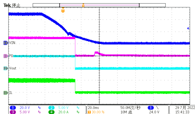
Figure 43. Power down(Iload=20A)
