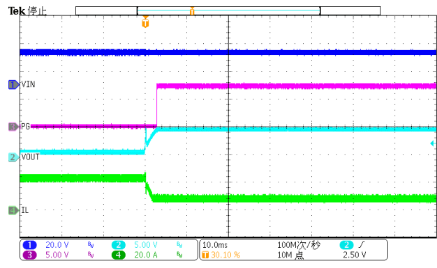
Figure 47. Hard Short Recovery
