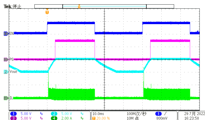
Figure 45. Enable (Iload=0.1A)
