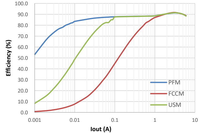
Figure 4. Efficiency, V_{in}=24V , V_{out}=5V , F_{sw}=400kHz
