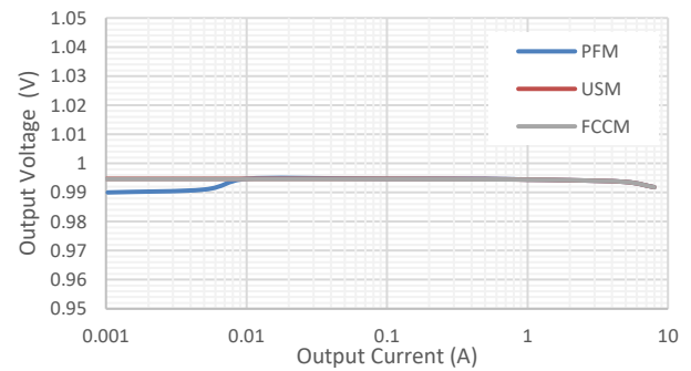
Figure 5. Load Regulation, VIN=5V, Vout=1V, Fsw=800kHz
