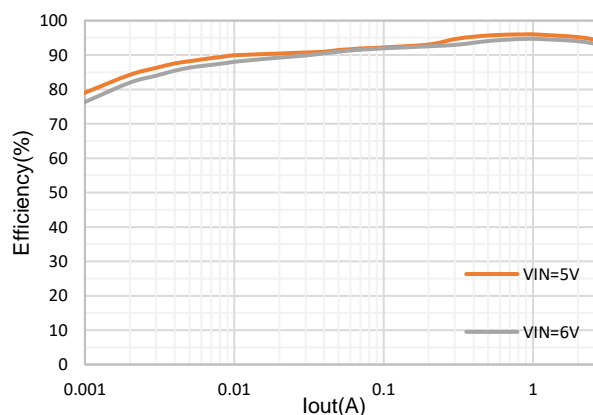
Efficiency, Vout=3.3V
