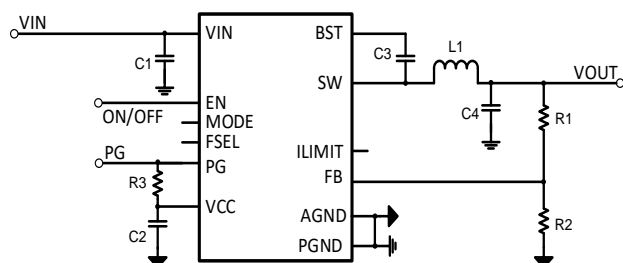
2.9V-7V, Synchronous Buck Converter
