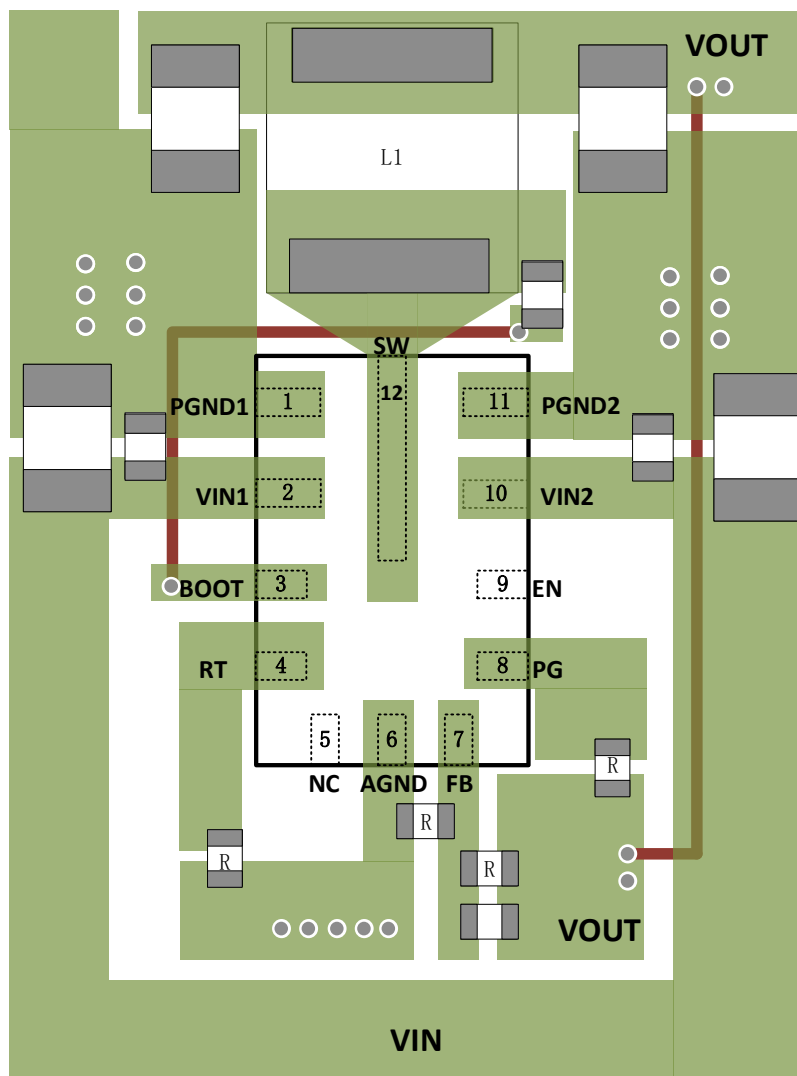
Figure 24. PCB Layout Example
