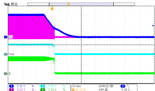
Figure 13. Power down( I_{LOAD}=3A )
