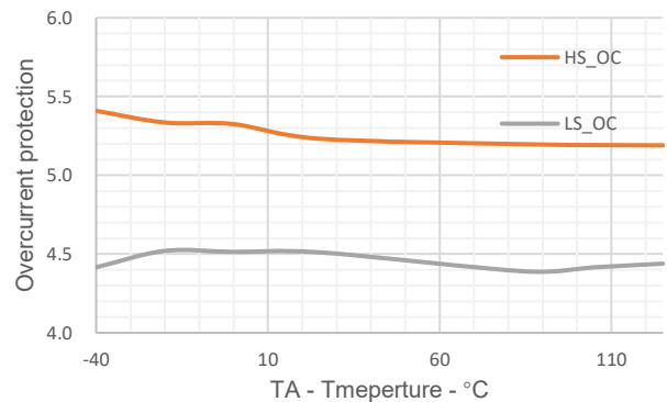
Figure 7. Current Limit vs Temperature
