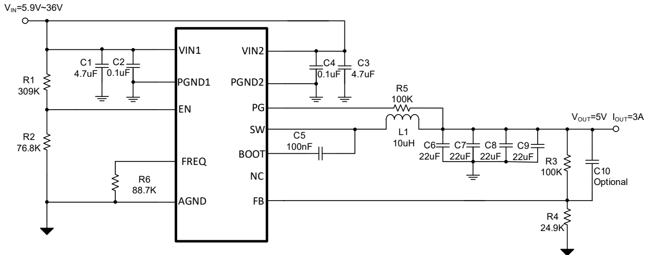
Figure 11. SCT2434DQ Design Example, 5V Output with Adjustable UVLO
