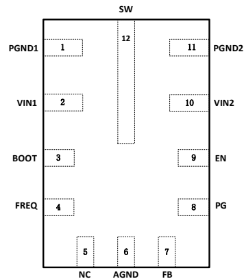
Figure 1. 12-Lead QFN 2mmx3mm
