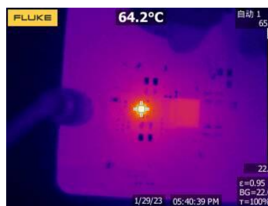
Figure 23. Thermal, 12V IN , 5V OUT , 3A
