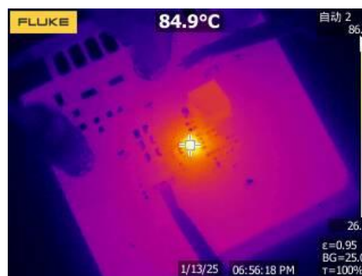
Figure 23. Thermal, 48VIN, 5VOUT, 2A
