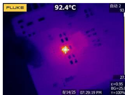
Figure 23. Thermal, 48VIN, 5VOUT, 1.5A
