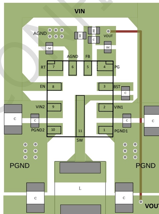
Figure 24. PCB Layout Example
