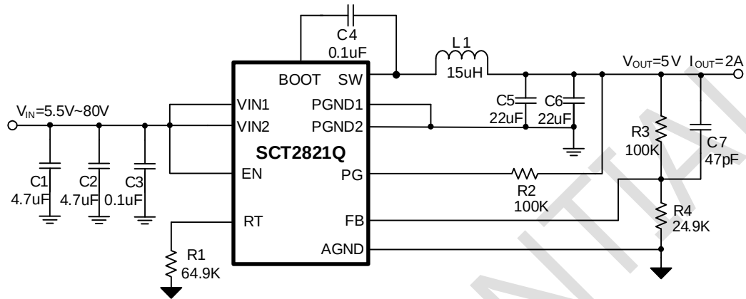
Figure 11. SCT2821Q Design Example, 5V Output
