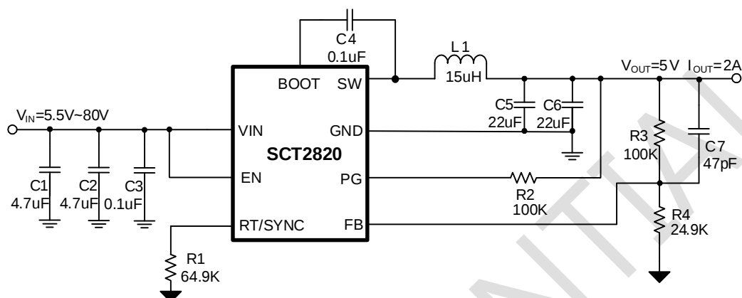
Figure 11. SCT2820 Design Example, 5V Output
