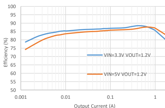
Efficiency at VOUT=1.2V
