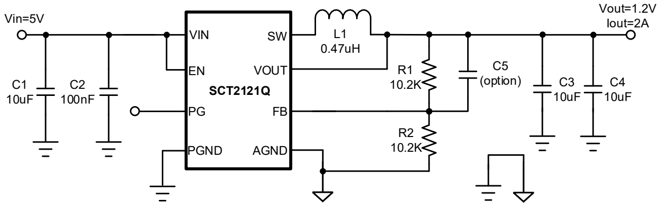
Figure 8. SCT2121Q Design Example, 1.2V Output
