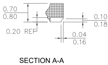
FCTQFN1.5X2-8L Package Outline Dimensions
