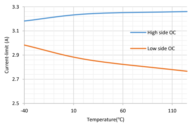
Figure 4. Current-limit vs Temperature
