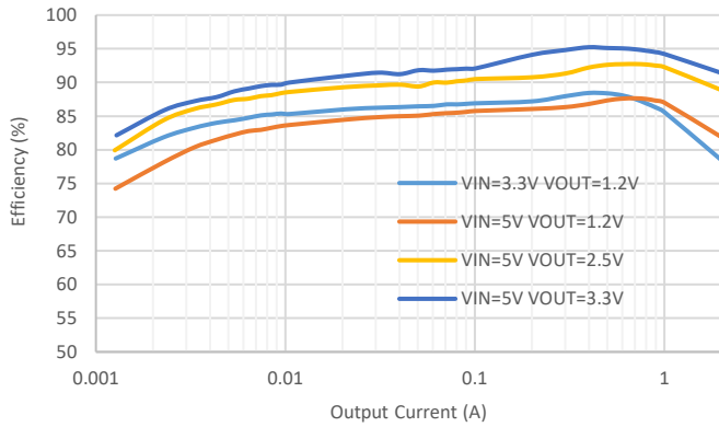
Figure 1. Efficiency vs Load Current
