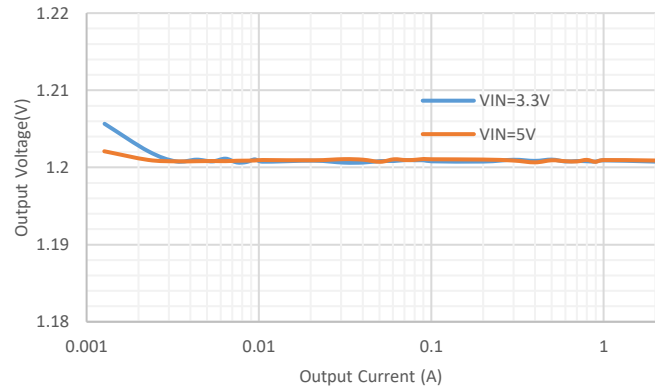
Figure 2. Load Regulation
