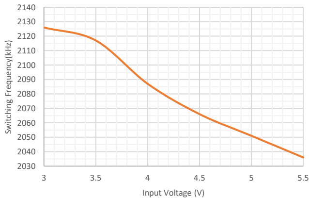
Figure 3. Frequency vs Input Voltage
