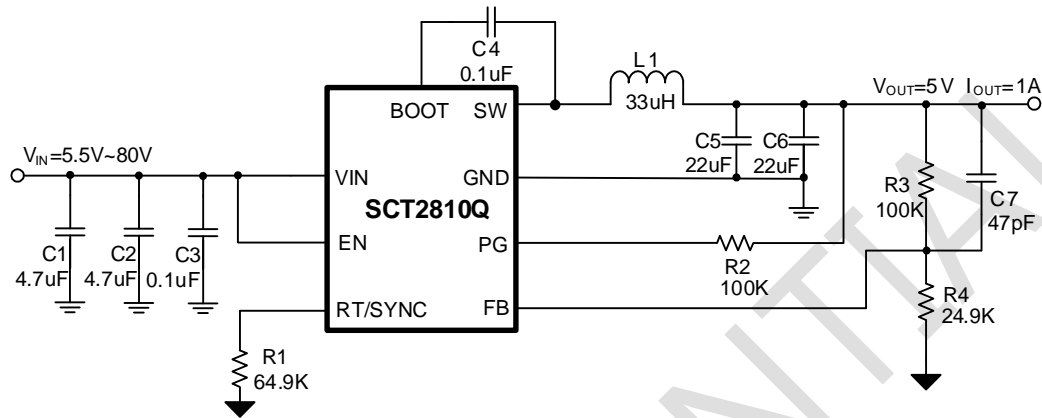
Figure 11. SCT2810Q Design Example, 5V Output
