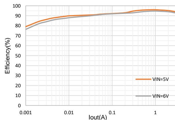
Efficiency, Vout=3.3V
