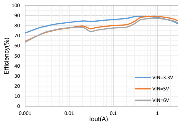
Figure 1. Efficiency vs Load Current, Vout=1.2V
