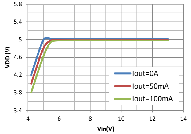
Figure 3. 5V LDO Vout vs Vin
