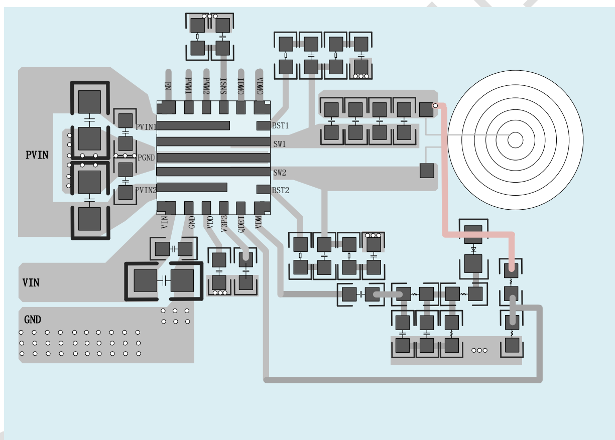
Figure 18. PCB Layout Example
