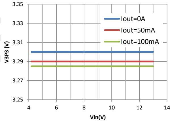
Figure 5. 3.3V LDO Vout vs Vin
