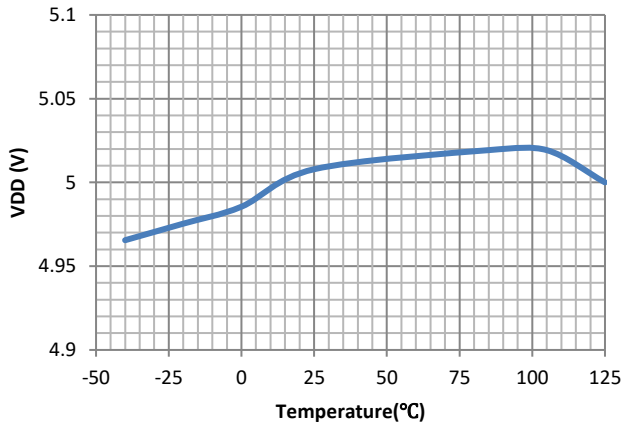
Figure 4. 5V LDO Vout vs temperature @ Vin = 9V
