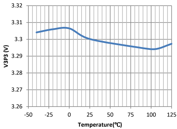
Figure 6. 3.3V LDO Vout vs temperature @ Vin = 9V
