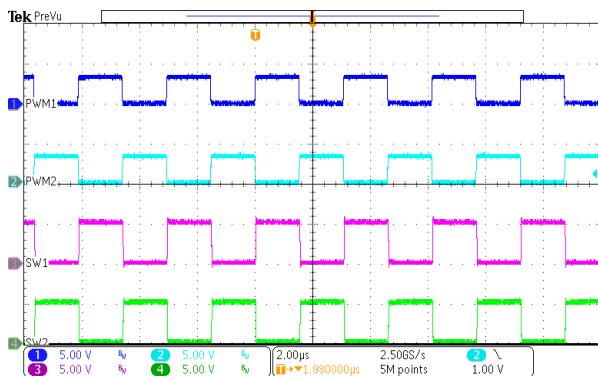
Figure 16. Full bridge @ V_{in}=5V , R_X=2.5W
