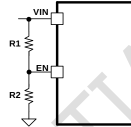
Figure 9. System UVLO by enable divide
