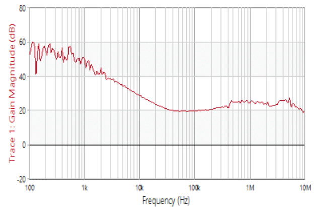
LDO PSRR, V_{OUT4}=2.8V , I_{OUT4}=100mA
