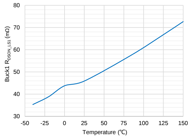
Buck1 R DSON_LS1 vs. Temperature
