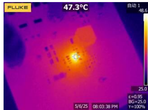
Figure 23. Thermal, 48V IN , 5V OUT , 1A
