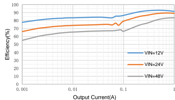
Efficiency, F sw =400kHz, V out =5V
