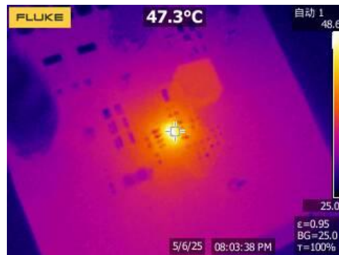
Figure 23. Thermal, 48V IN , 5V OUT , 1A
