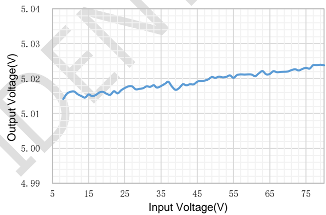
Figure 5. Line Regulation ( V_{out}=5V , I_{load}=1A )
