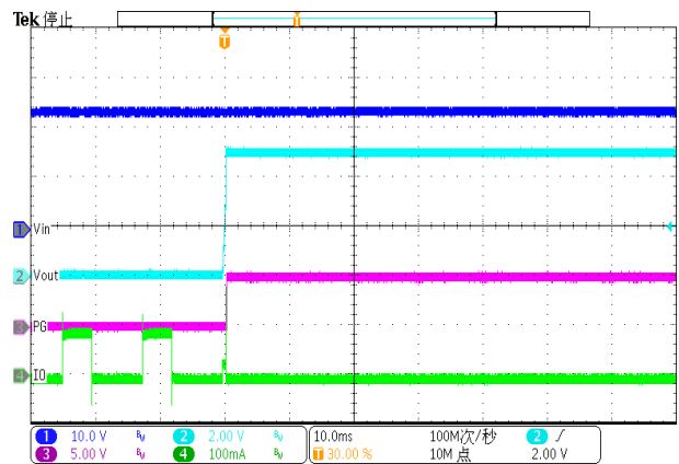
Figure 59. Exit Over Temperature Protection
