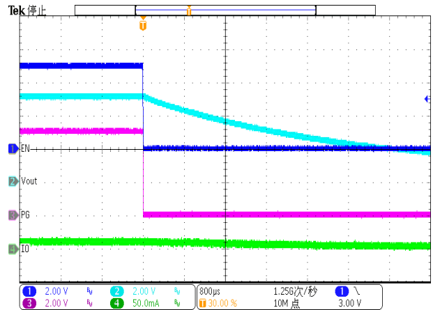
Figure 47. Disable (Iload=10mA)
