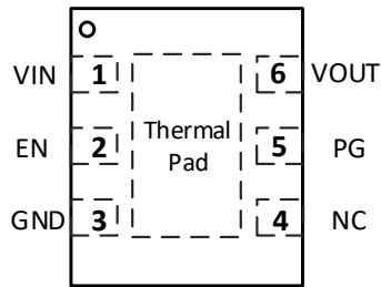
SCT71403FxxAQDVAR TQFN2X2-6L Package
