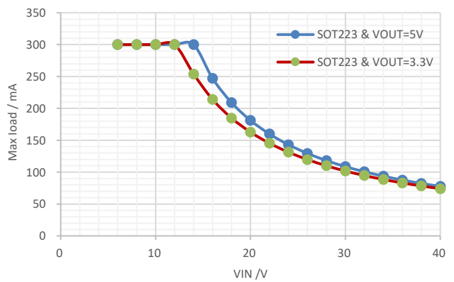
Figure 41. Maximum Output Current vs Input Voltage, SOT223-4L, T_J \leq 150^\circ\text{C}
