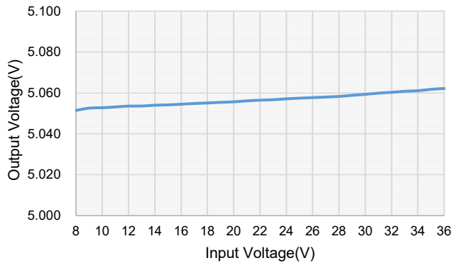
Figure 4. Line Regulation ( F_{sw}=400kHz , V_{out}=5V )
