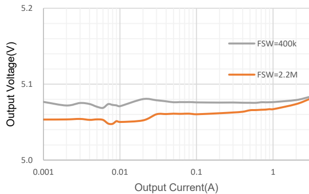
Figure 6. Load Regulation ( V_{in}=12V , V_{out}=5V )
