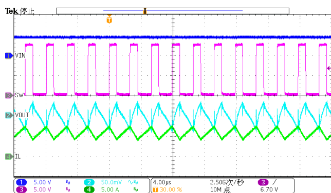
Figure 27. Steady-state (Iload=2A)
