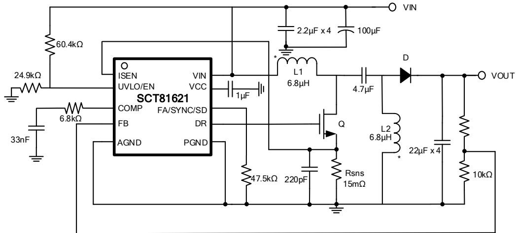
Figure 29. Application Schematic, 5V to 50V, 2A Sepic Regulator at 400kHz
