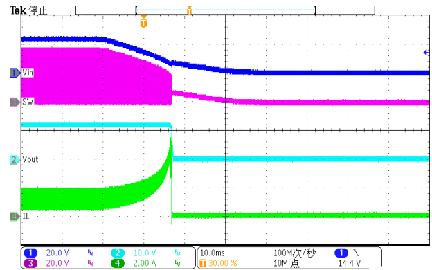
Figure 32. Power down(Iload=2A)
