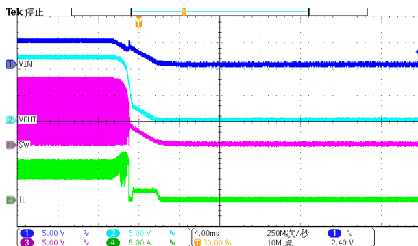
Figure 24. Power down(Iload=2A)
