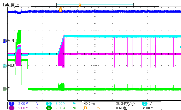
Figure 26. Over current recovery (Iload=5A)
