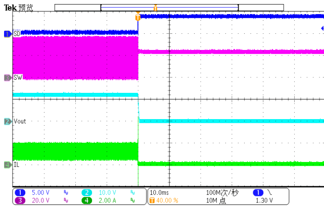
Figure 33. Shutdown entry
