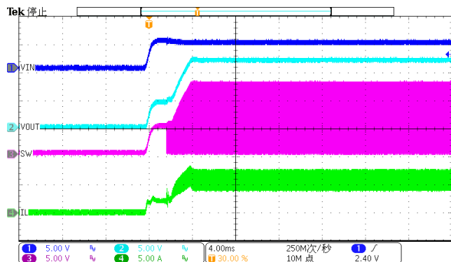
Figure 23. Power up(Iload=2A)
