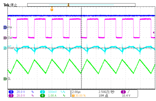
Figure 36. steady-state (Iload=2A)
