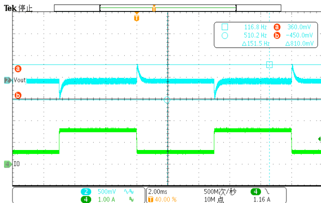
Figure 35. LoadTrans (Iload=0.5A-1.5A)
