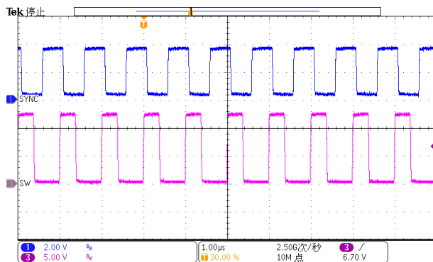
Figure 28. Sync Frequency
