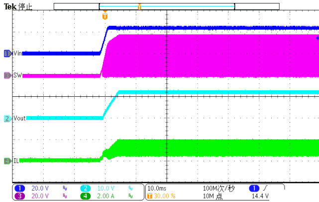
Figure 31. Power up(Iload=2A)
