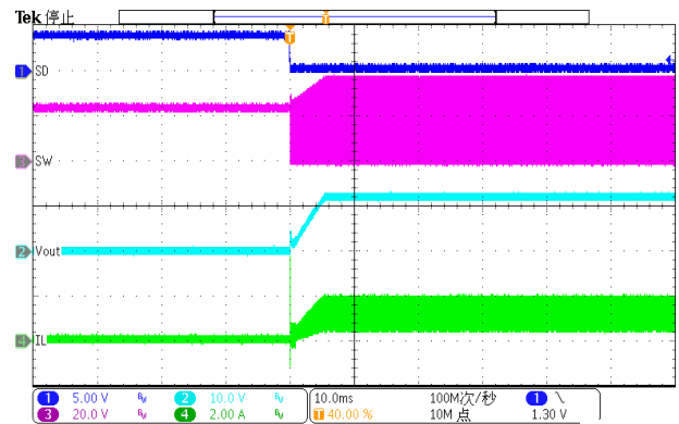
Figure 34. Shutdown remove
