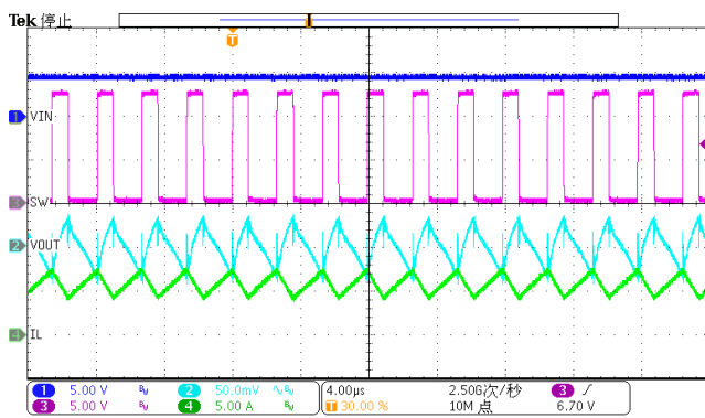
Figure 26. Steady-state (Iload=2A)
