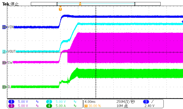
Figure 22. Power up(Iload=2A)
