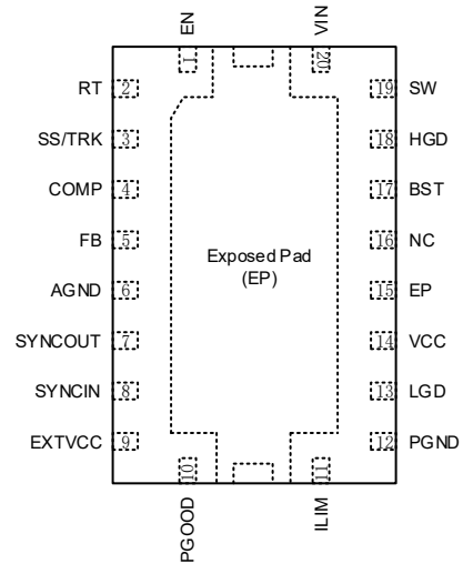
Top View: DFN3.5X4.5-20L
