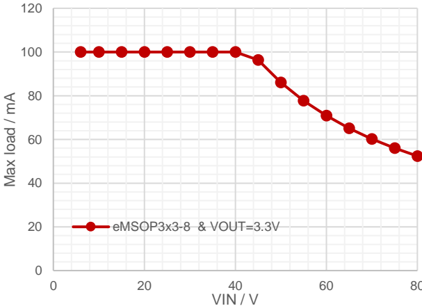
Figure 29. Maximum Output Current vs Input Voltage, VOUT=3.3V of EMSOP-8L, T_J \leq TSD\_R
