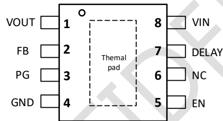
SCT71801A00MTER EMSOP-8L Package
