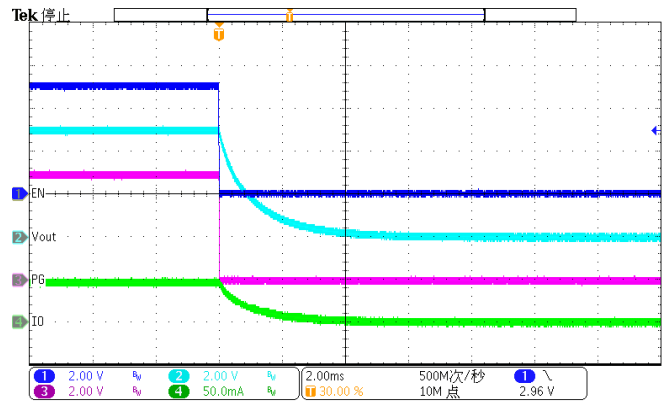
Figure 39. Disable (Iload=50mA)
