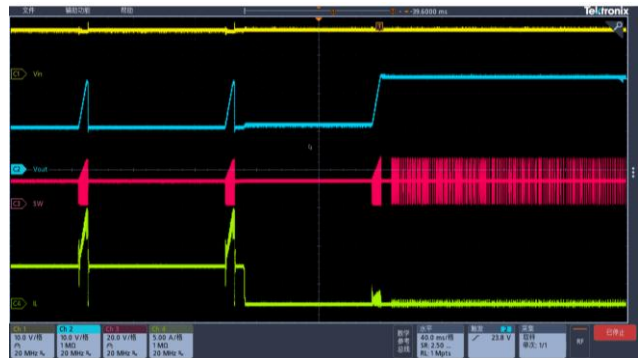
Figure 25. Over current recovery ( I_{LOAD}=5A )
