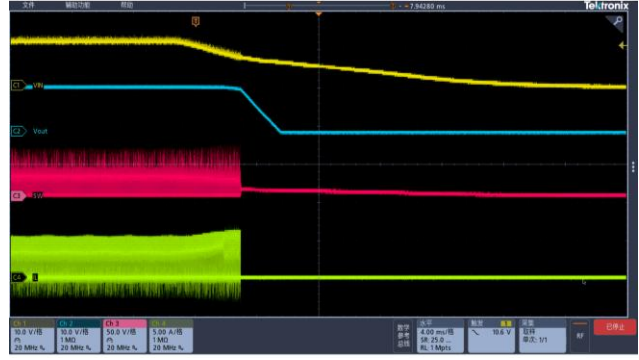
Figure 32. Power down ( I_{LOAD}=2A )
