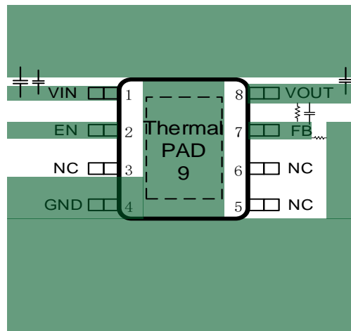
Figure 39. PCB Layout Example
