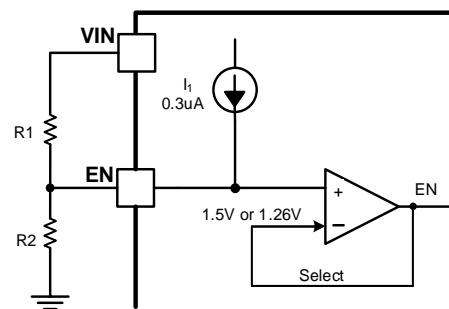
Figure 14. System UVLO by enable divide
