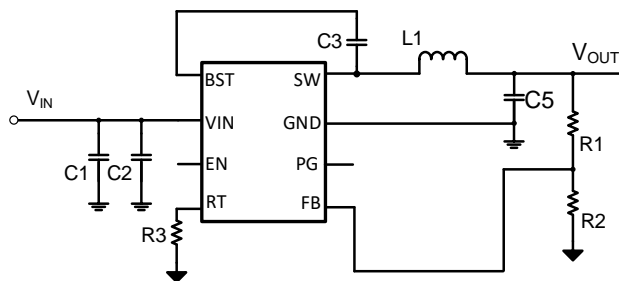
3.8V-30V, Synchronous Buck Converter Simplified schematic diagram
