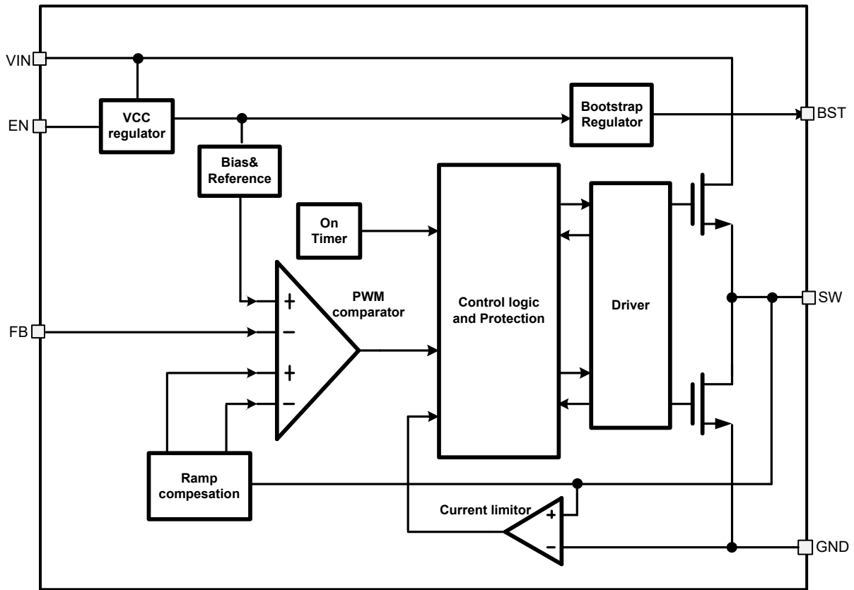
Figure 7. Functional Block Diagram
