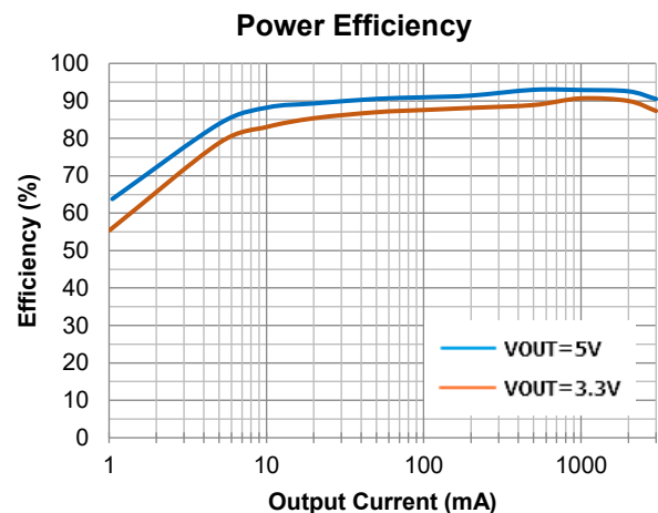
Efficiency, Vin=12V
