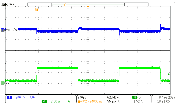
Figure 13. Load Transient VOUT=3.3V, IOUT=0.3A to 2.7A, SR=250mA/us
