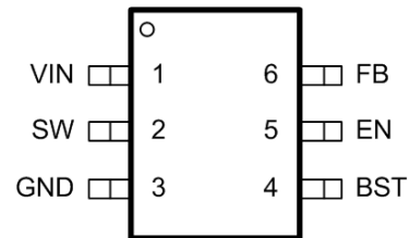
SOT563 Top View (1.6mm x 1.6mm)
