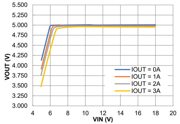
Figure 2. VOUT Vs. VIN
