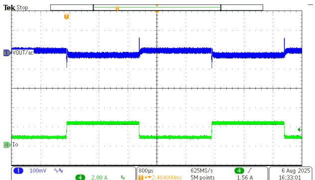
Figure 14. Load Transient VOUT=3.3V, IOUT=0.75A to 2.25A, SR=250mA/us
